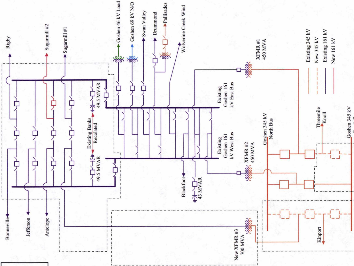
Goshen 345/161 kV Transformer Installation One-line
